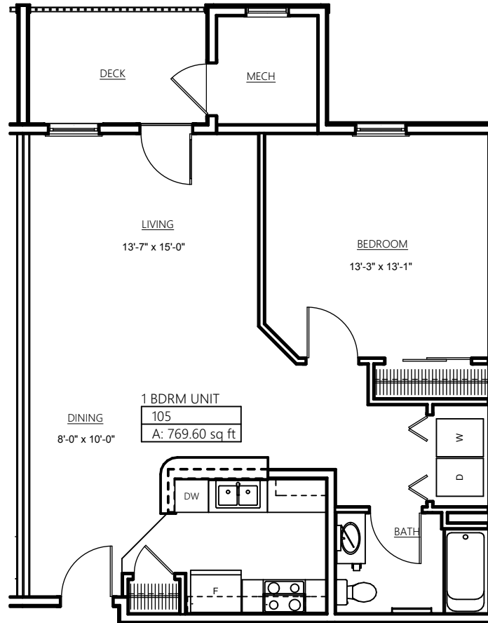
ONE BEDROOM UNIT NTS
