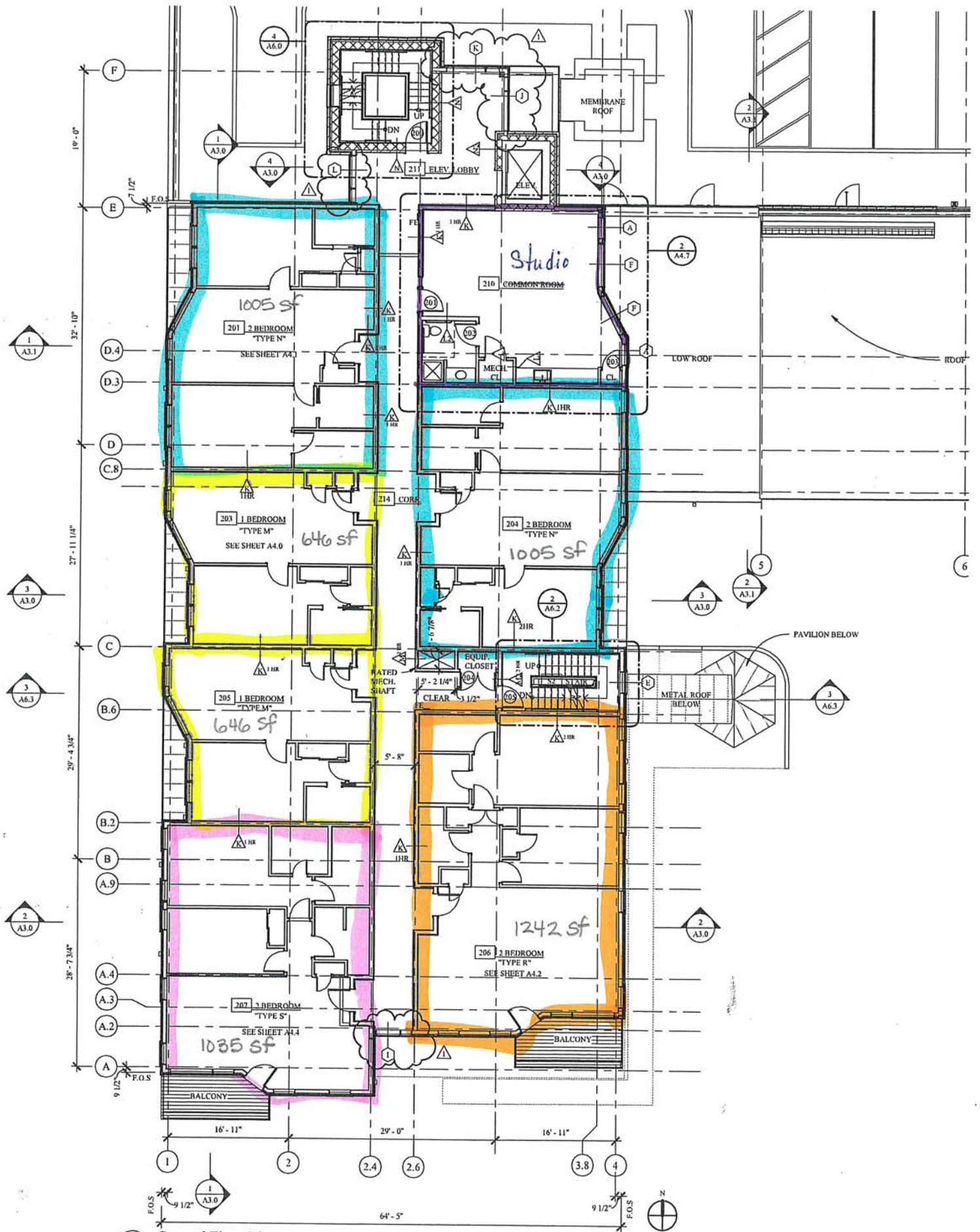
1 Second Floor Plan 1/8" = 1'-0"
