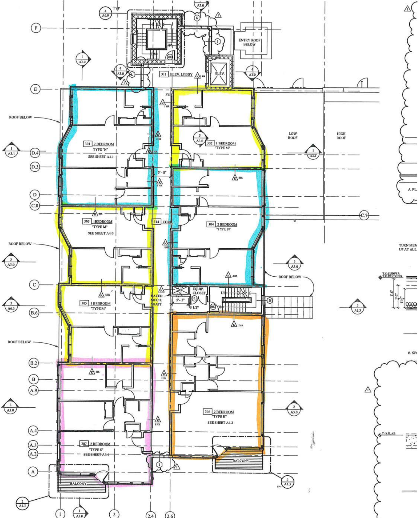
1 Third Floor 1/8" = 1'-0" Floor Plan
